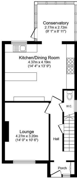
Ground Floor Floor area 54.1 sq.m. (583 sq.ft.)
